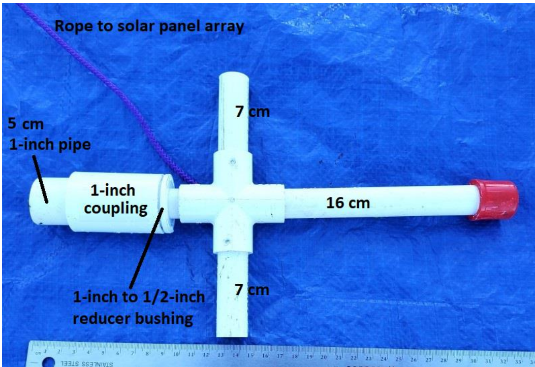
The power connector is constructed from \frac{1}{2} -inch PVC pipe. Flotation is added inside the pipe and 1-inch coupling.
