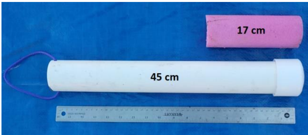
The float is constructed from 1 ½-inch PVC pipe.
