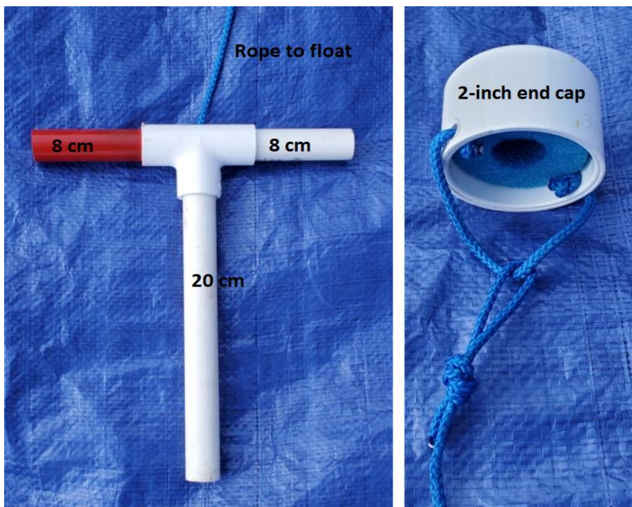
Left: The Eco-Mooring is constructed from ½-inch PVC pipe. Right: The float of the Eco-Mooring. The rope should be long enough so the float is on the surface when the Eco-Mooring is deployed into the base.
