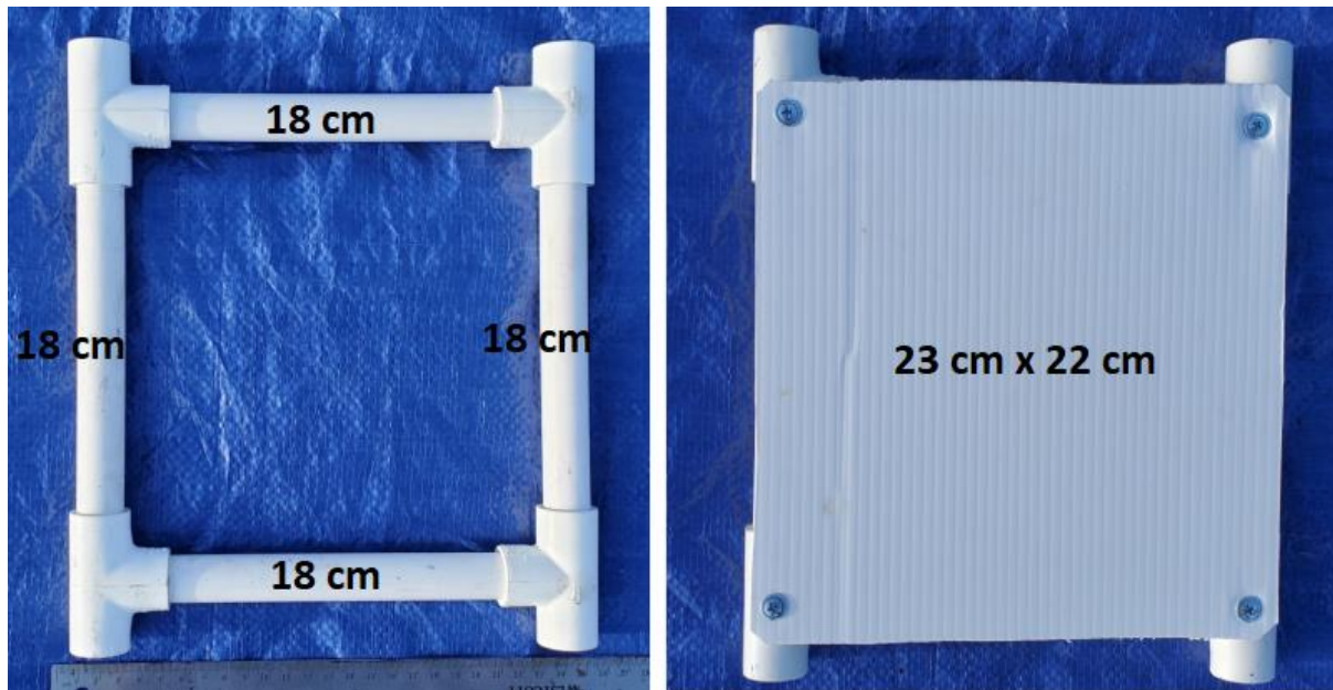
Left: The framework for the seagrass image is constructed from ½-inch PVC pipe. Right: A 23 cm x 22 cm rectangle of corrugated plastic sheeting is attached to the framework.
