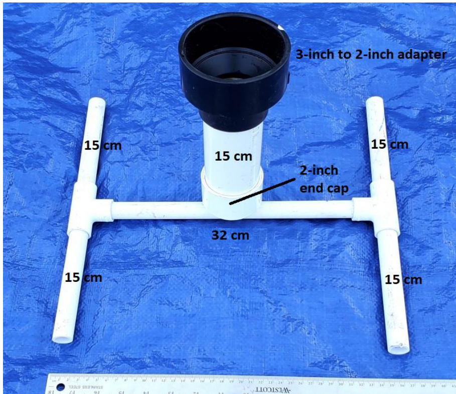
The Eco-Mooring base framework is constructed from ½-inch PVC.
