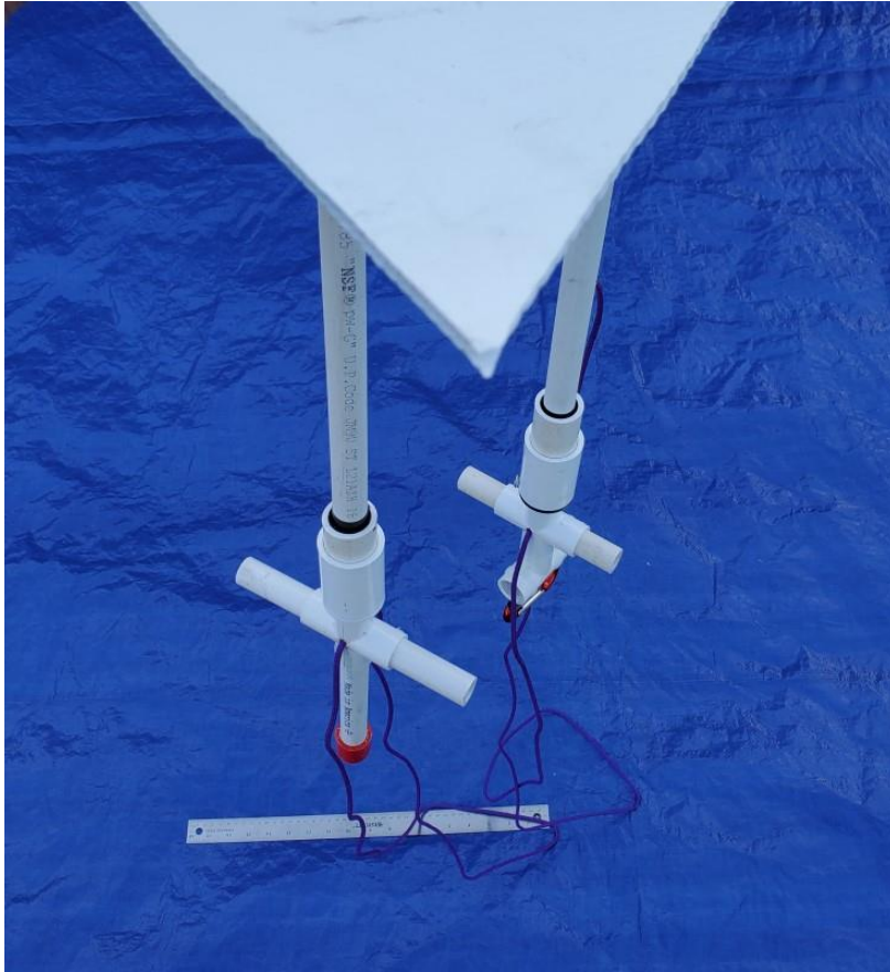
The mooring connector and power connector attached to the solar panel array.
