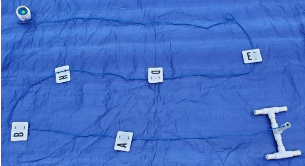
The buoy rope with base and lettering. At the world championship competition, in shallow water, the buoy rope will be deployed at an angle. A separate rope will descend from the buoy to a weight on the bottom which is offset from the base of the buoy rope.
