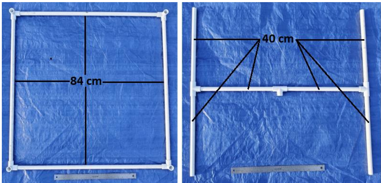
Left: The base of the docking station constructed from 1/2-inch PVC pipe. Right: The rear of the docking station constructed from 1/2-inch PVC pipe.
