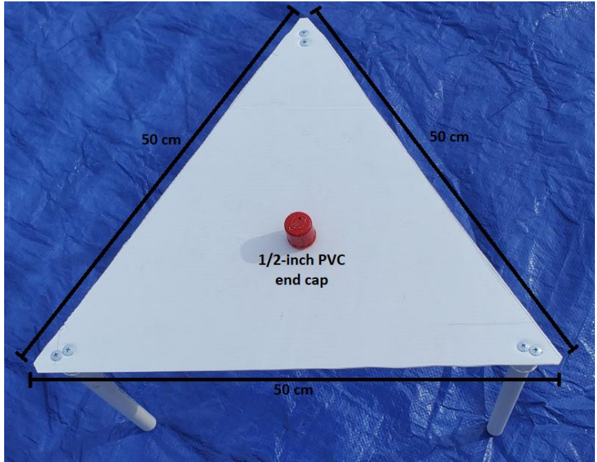
The solar panel array is constructed from corrugated plastic sheeting .
