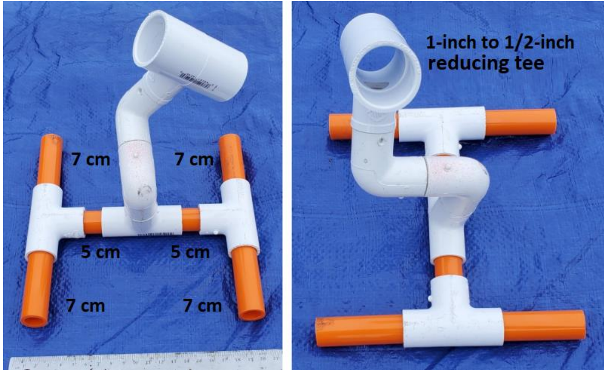
Left: Camera front view constructed from ½-inch PVC pipe. Right: Camera side view.
