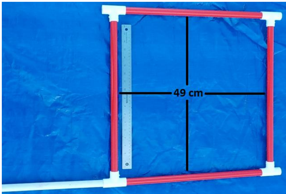
The area to deploy the vertical profiling float is constructed from ½-inch PVC pipe. At the World Championship, PIONEER class companies will deploy their floats at the edge of the deep end of the pool.
