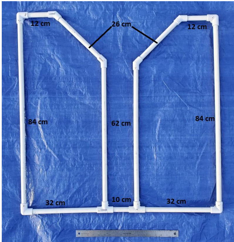
The top of the docking bay constructed from 1/2-inch PVC pipe.
