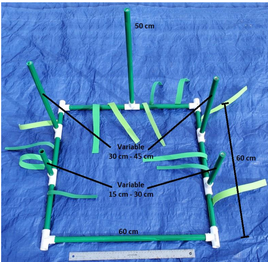
A release site framework constructed from ½-inch PVC pipe with 30 cm lengths green foam sheeting .
