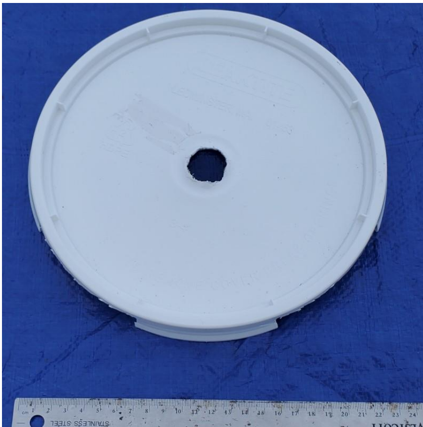
A 2-gallon bucket lid. The hole in the center is large enough for the threaded end of the 3/4-inch male adapter to fit through.
