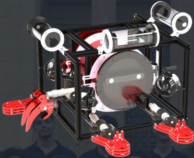
Figure1. : GLACIUS , Rendered from Solidworks by Nour hassanein
