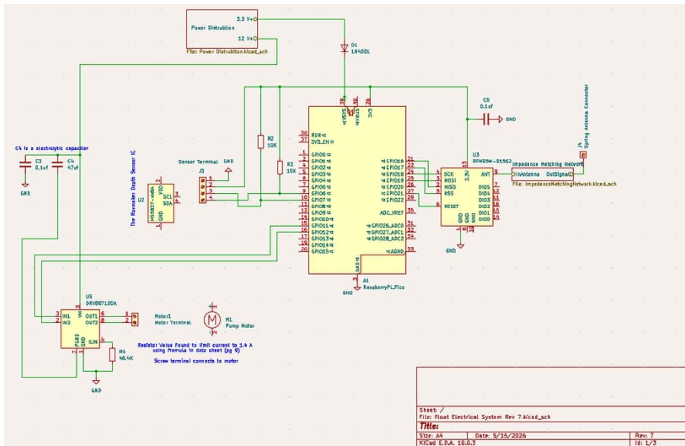
Figure 7 Detailed PCB diagram & SID
