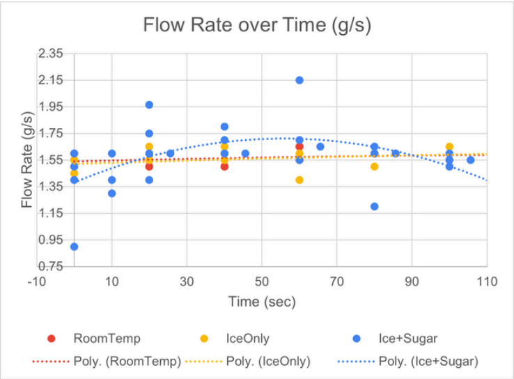
Figure 4: Flow rate vs. time graph
