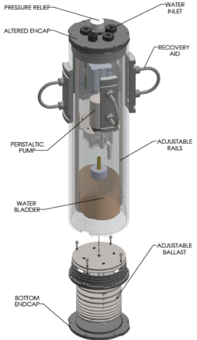
Figure 1: Assembled float in Solidworks CAD software
