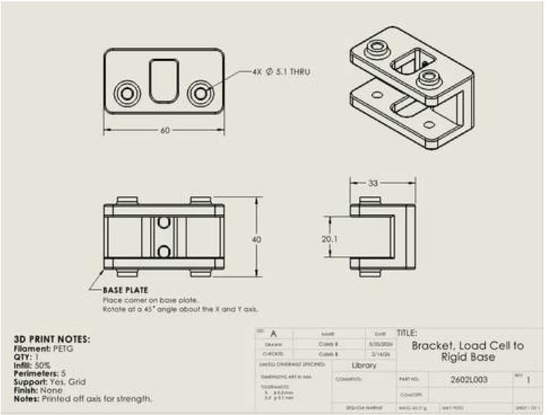
Figure 6: Sample of a drawing intended for 3D printing
