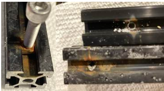
Figure 37: Corrosion testing, salt v. freshwater test
