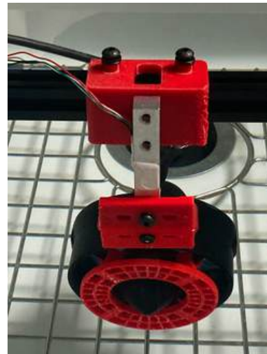
Figure 39: Load cell thrust testing of shrouds
