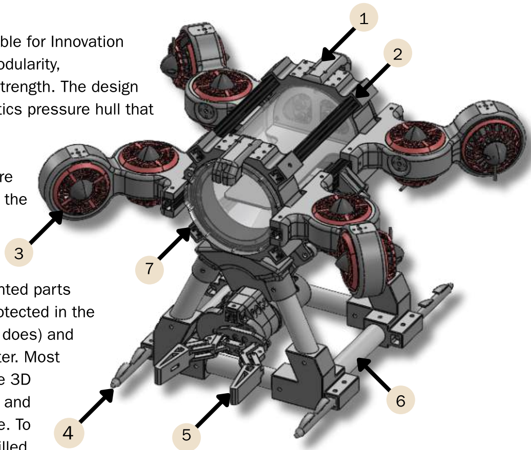
Figure 3: ROSIE the ROV fitted with all components
