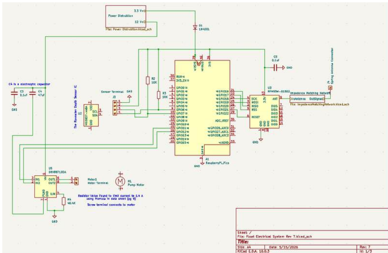
Figure 32: Detailed PCB diagram & SID
