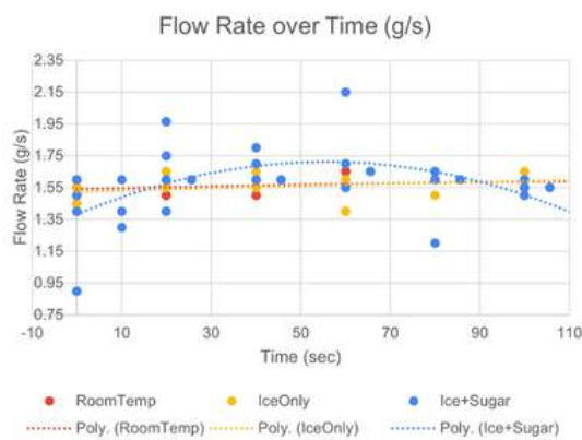
Figure 29: Flow Rate vs Time Graph (left)
