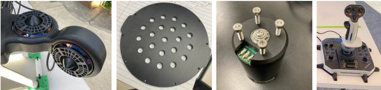
Figure 36: Thruster mounts, backplate, DD3130 motor, flight stick
