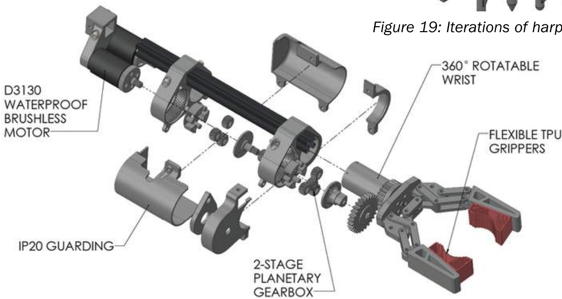
Figure 20: Explode view of SMS's 2 DOF Manipulator
