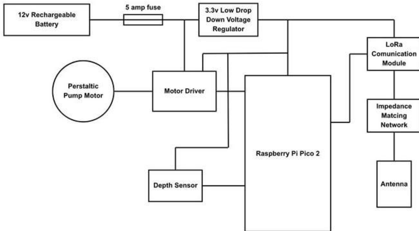
Figure 33: Simplified SID diagram
