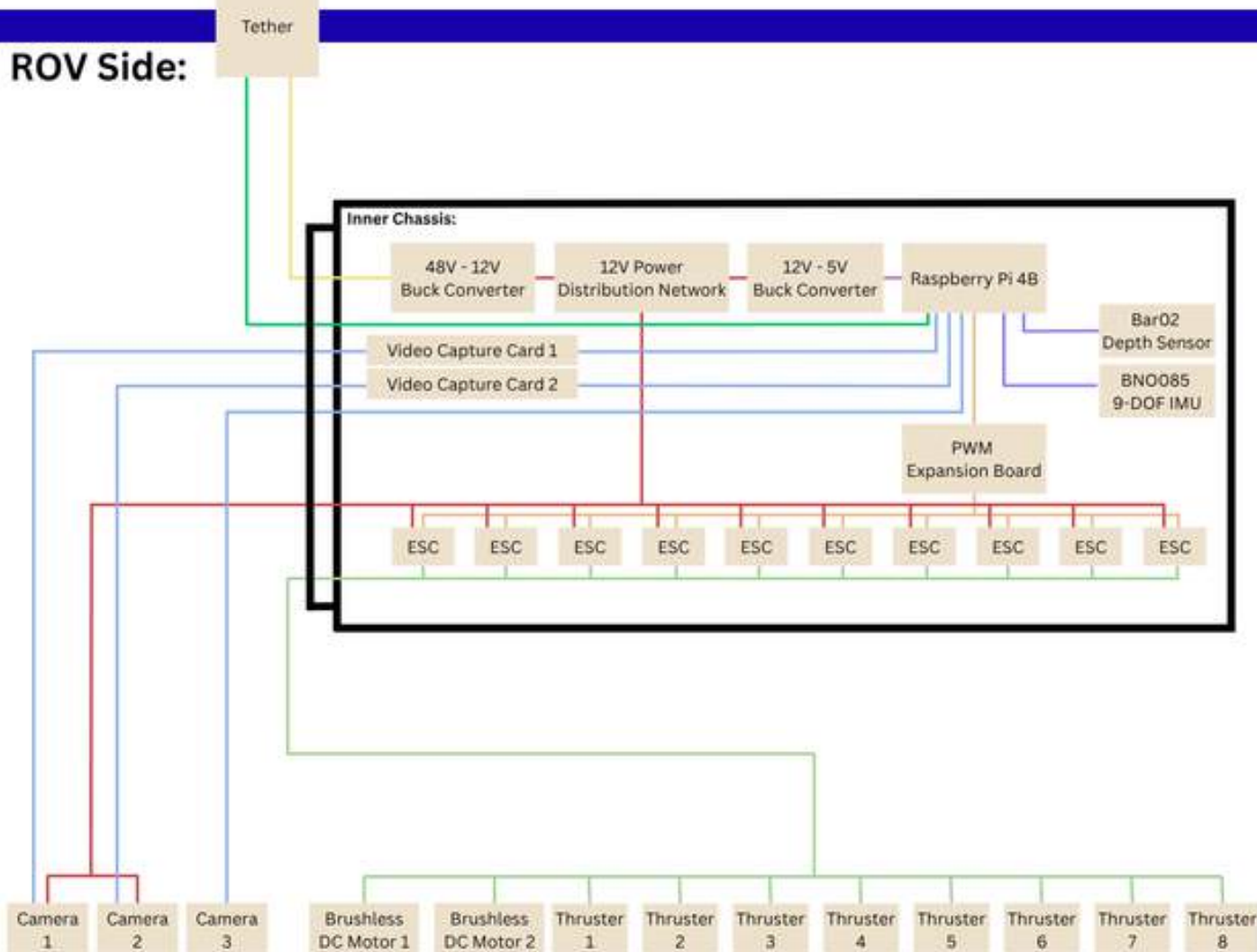
Figure 34: Simplified SID diagram
