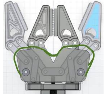
Figure 21: Linkage guard iteration
