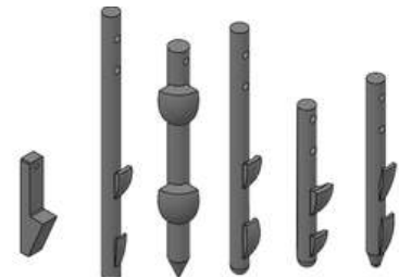
Figure 19: Iterations of harpoon (left to right)
