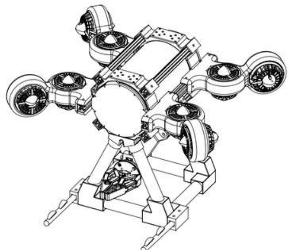
Figure 5: A prototype blueprint of ROSIE
