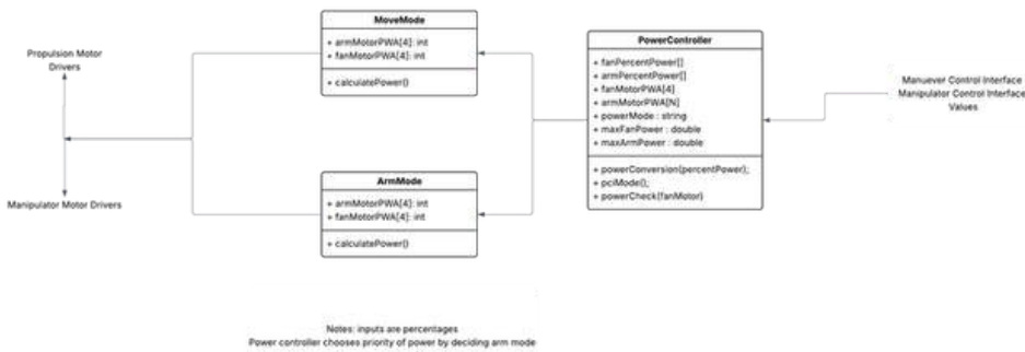
Figure 17: UML Class Diagram for the Power Control Interface subsection
