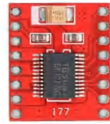
FIGURE 25: TB6612FNG MOTOR DRIVE BOARD
