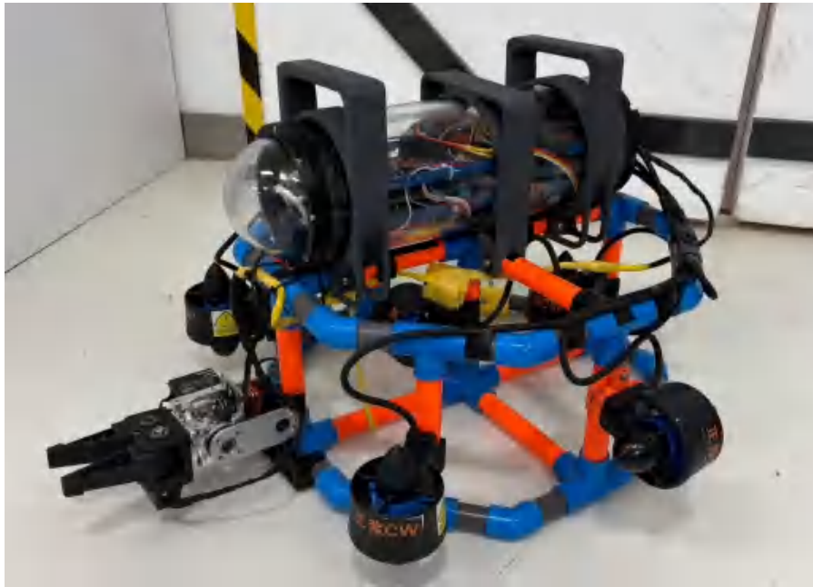
FIGURE 10: STRUCTURE IN REAL WORLD
