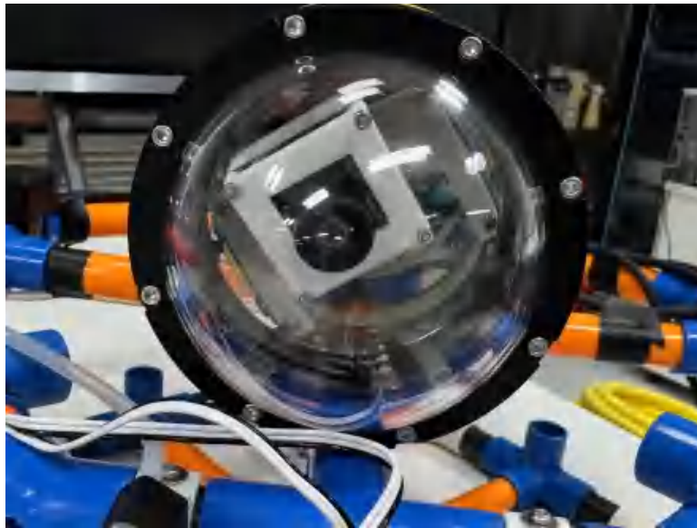
FIGURE 22: PANORAMIC CAMERA
