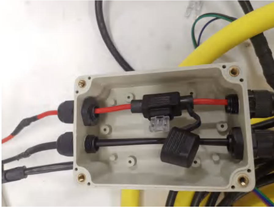
FIGURE 29: FUSE
