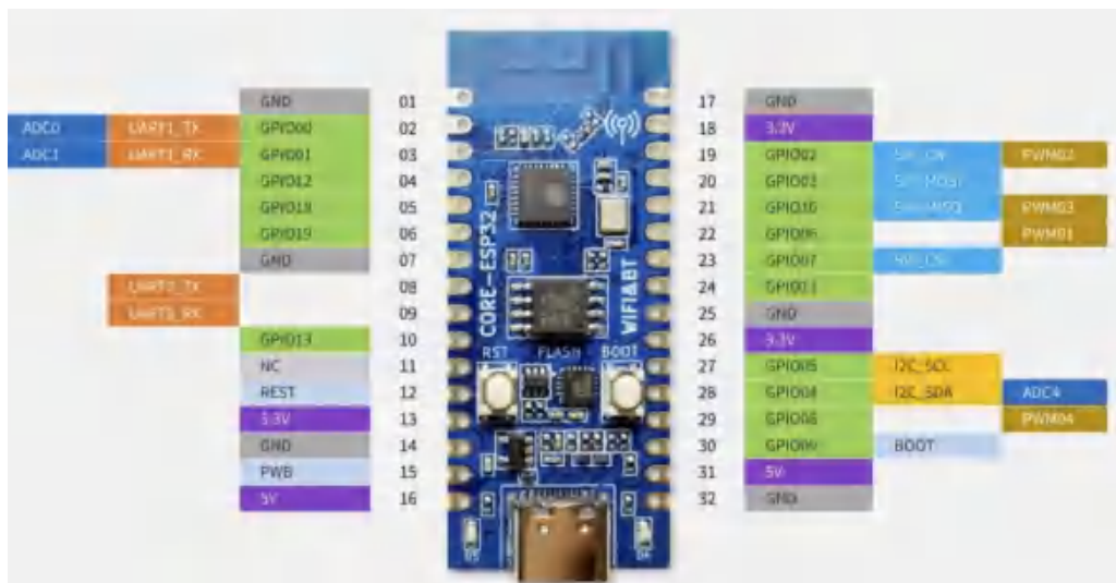
FIGURE 24: ESP32 MICROCONTROLLER
