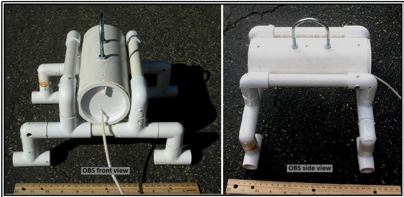
RANGER mission photo #17: OBS front view and OBS side view.
