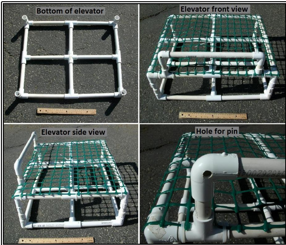
RANGER mission photo #15: Partial construction of elevator bottom, elevator front view, elevator side view, and view of hole for the pin.
