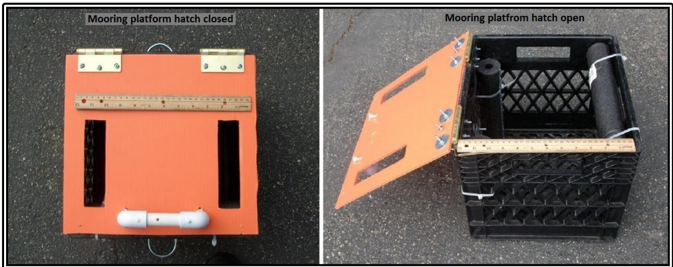
RANGER mission photo #25: Mooring platform with hatch closed and open. Mooring will be held in mid-water with four lengths of rope connected to weights.
