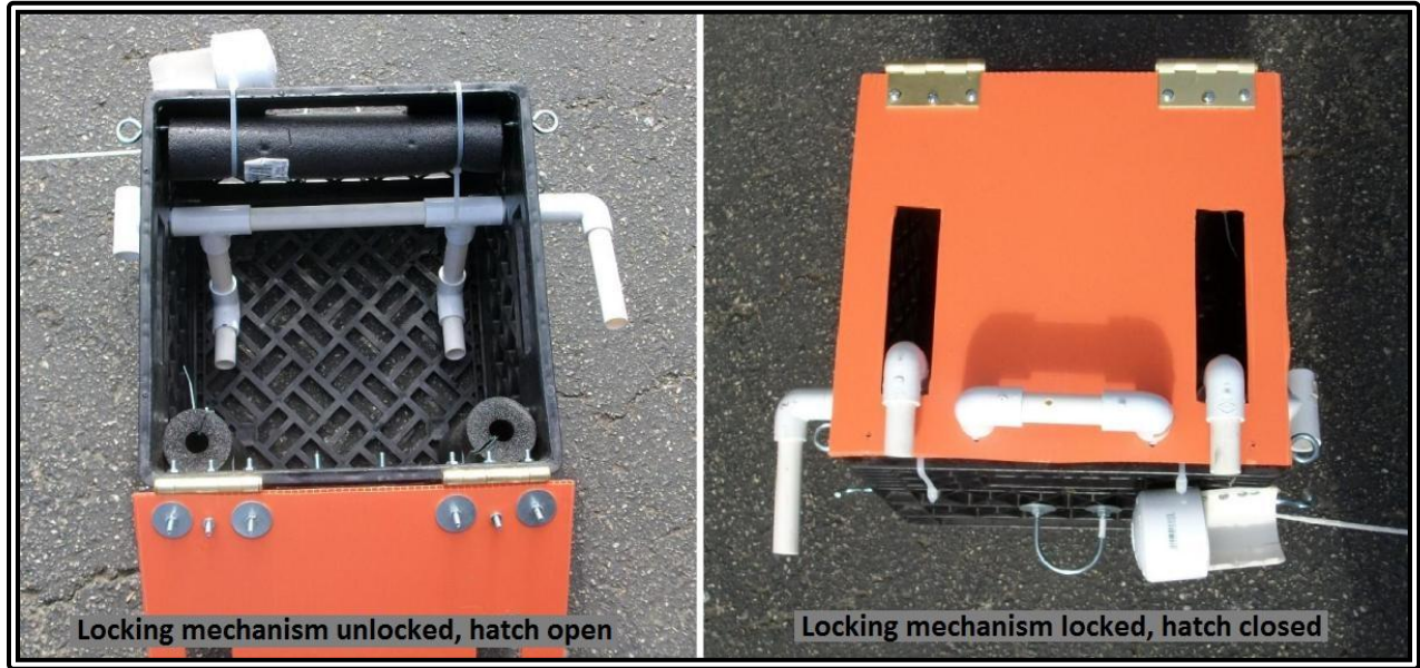
RANGER mission photo #27: Locking mechanism unlocked, hatch open and locking mechanism locked, hatch closed.
