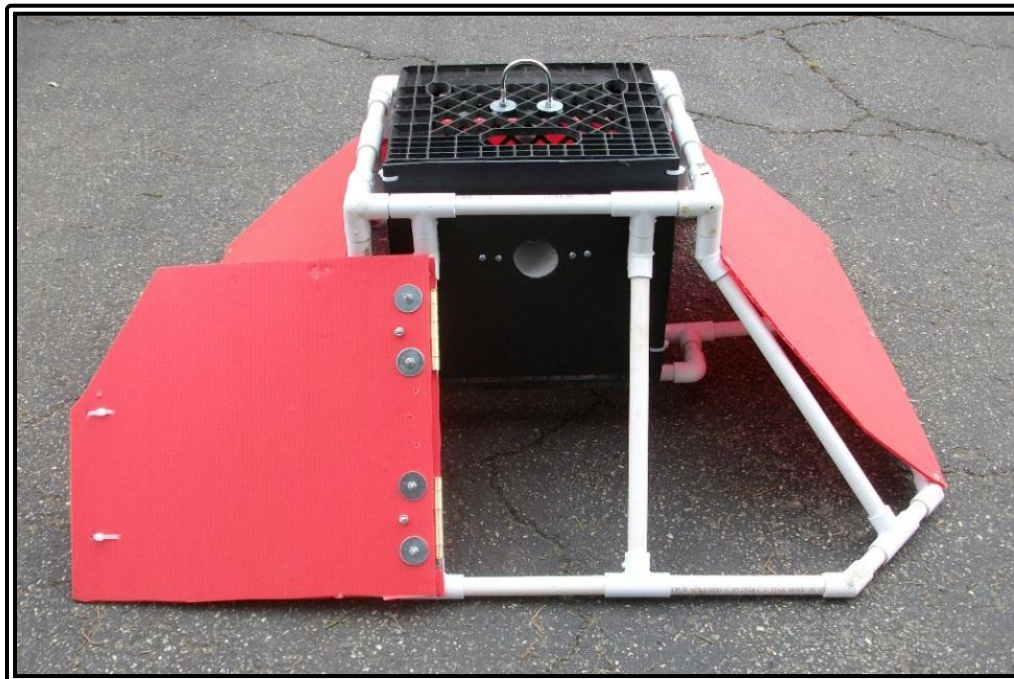
RANGER mission photo #10: SIA inside of BIA. Door open.
