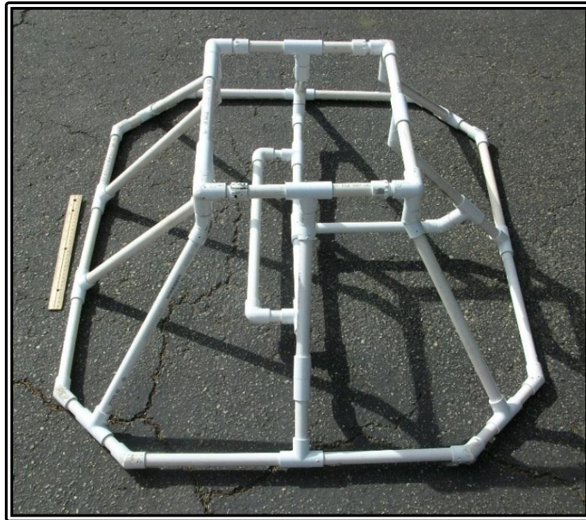
RANGER mission photo #3: Side view of BIA framework.
