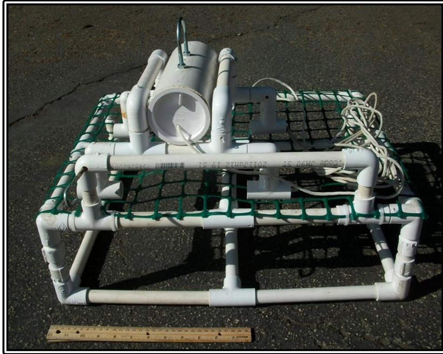
RANGER mission photo #19: Front view of elevator with OBS, OBS cable connector, and cable.
