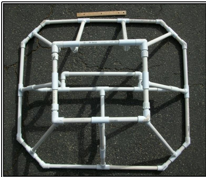
RANGER mission photo #4: Top view of BIA framework.
