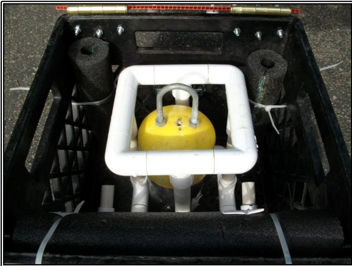
RANGER mission photo #30: ADCP inside cradle inside mooring platform.
