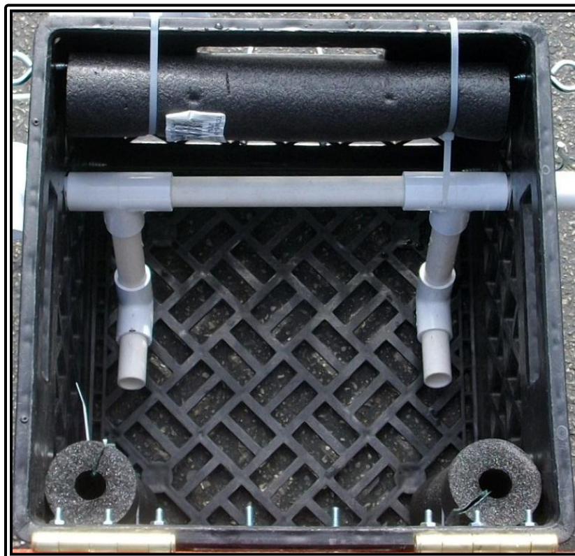
RANGER mission photo #34: Flotation for mooring platform.
