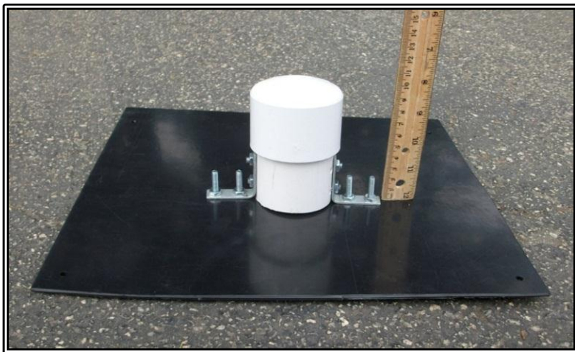
RANGER mission photo #8: Partial construction of SIA bulkhead connector (inner side).
