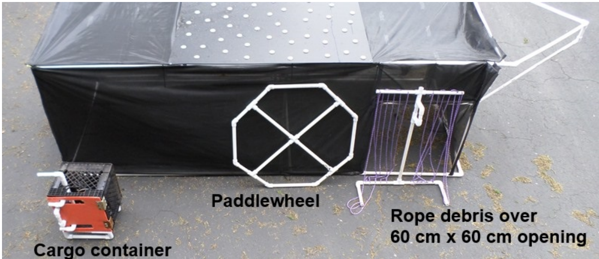
RANGER mission photo #1: The starboard side of shipwreck with cargo container, paddlewheel and rope debris over the 60 cm x 60 cm opening.
