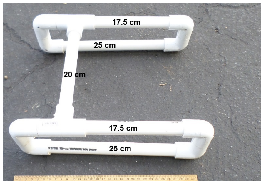
RANGER build photo #33: Stand for cargo container.
