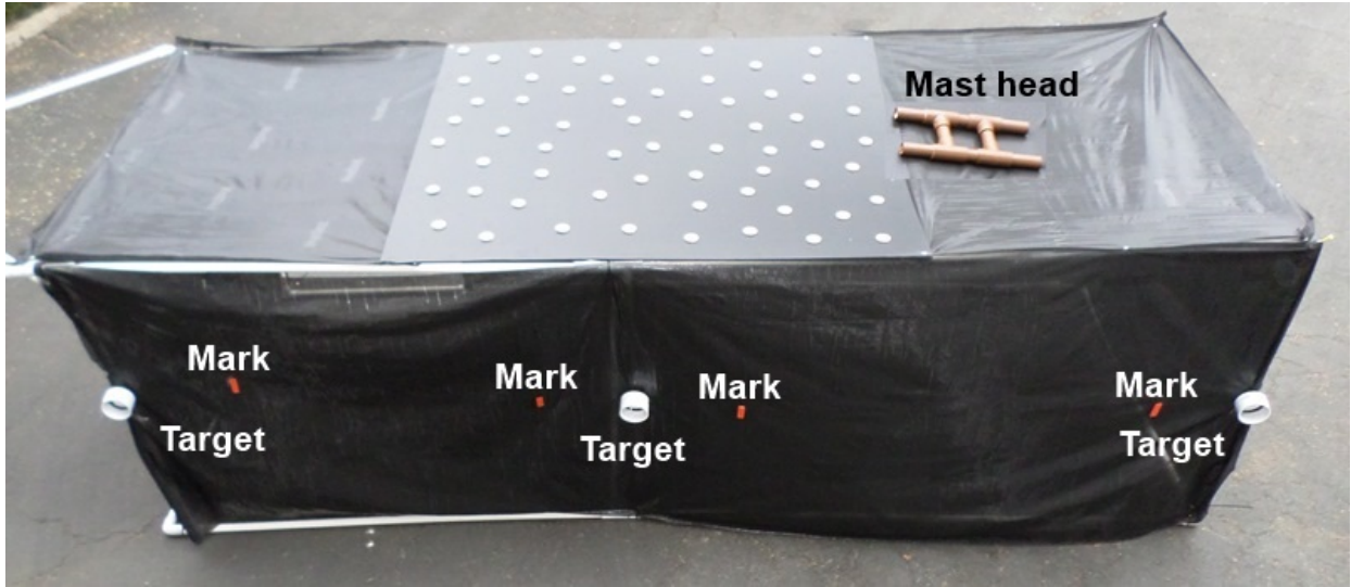
RANGER mission photo #3: The port side of the shipwreck with three scan targets and the mast head visible on the top of the shipwreck.
