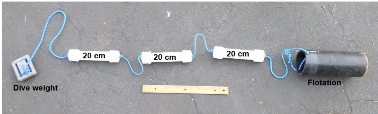
RANGER build photo #48: Sensor string.
