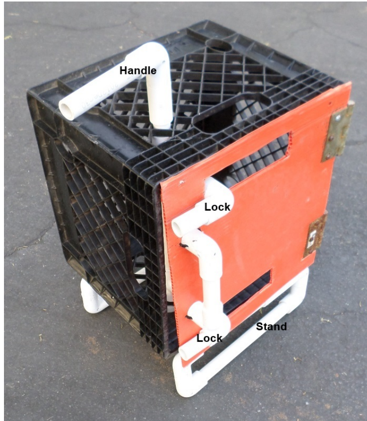
RANGER build photo #34: Cargo container, locked, on stand.
