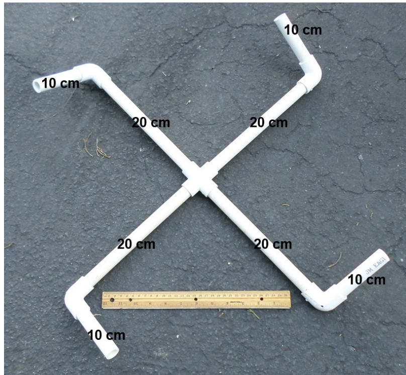
RANGER build photo #23: The framework of the propeller.
