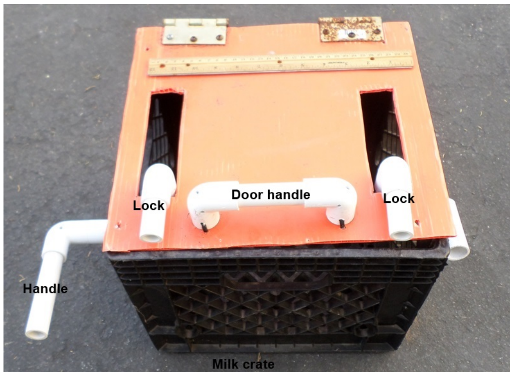
RANGER build photo #32: Cargo container, closed and locked.
