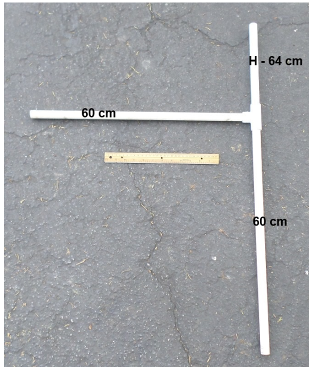
RANGER build photo #10: 60 cm x 60 cm opening components.
