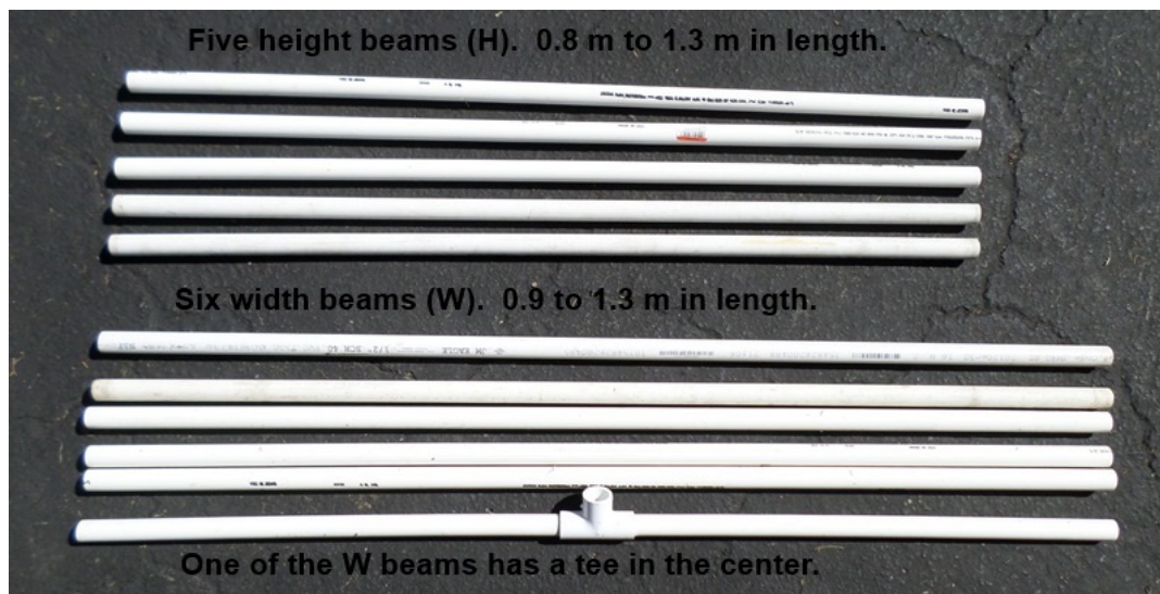
RANGER build photo #1: W and H beams.
