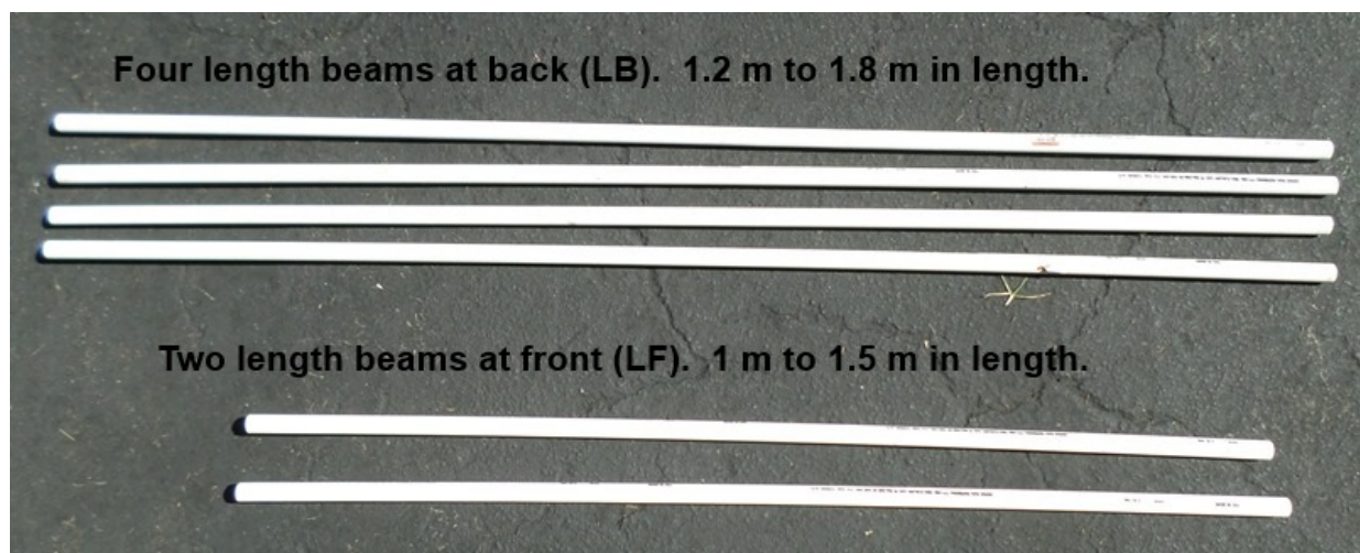
RANGER build photo #2: LF and LB beams.
