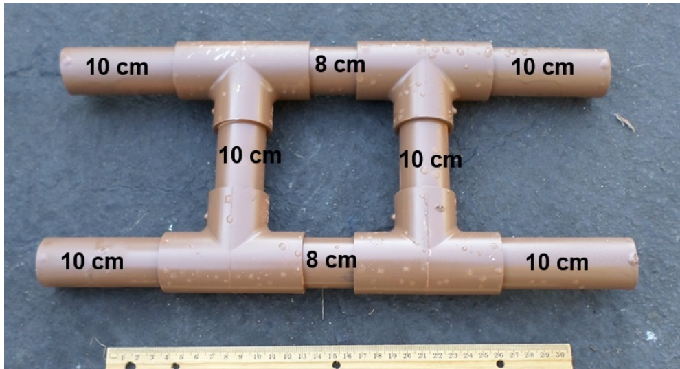
RANGER build photo #19: Mast head.
