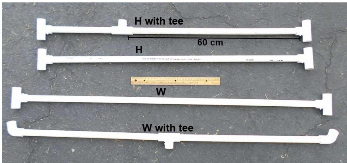
RANGER build photo #7: Components of bow cross section.
