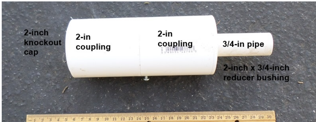
RANGER build photo #53: Simulated glass bottle.
