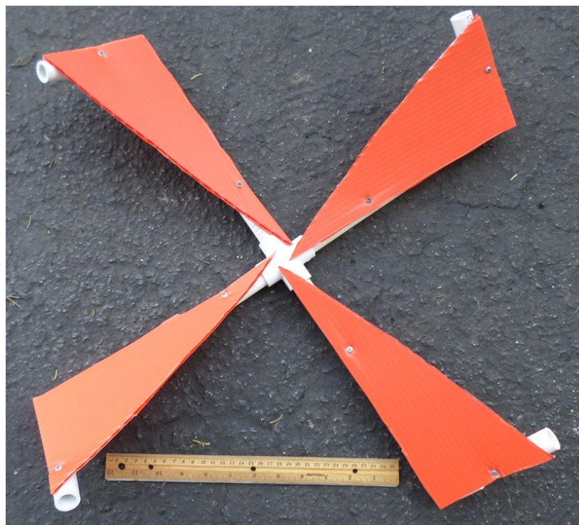
RANGER build photo #24: The propeller.
