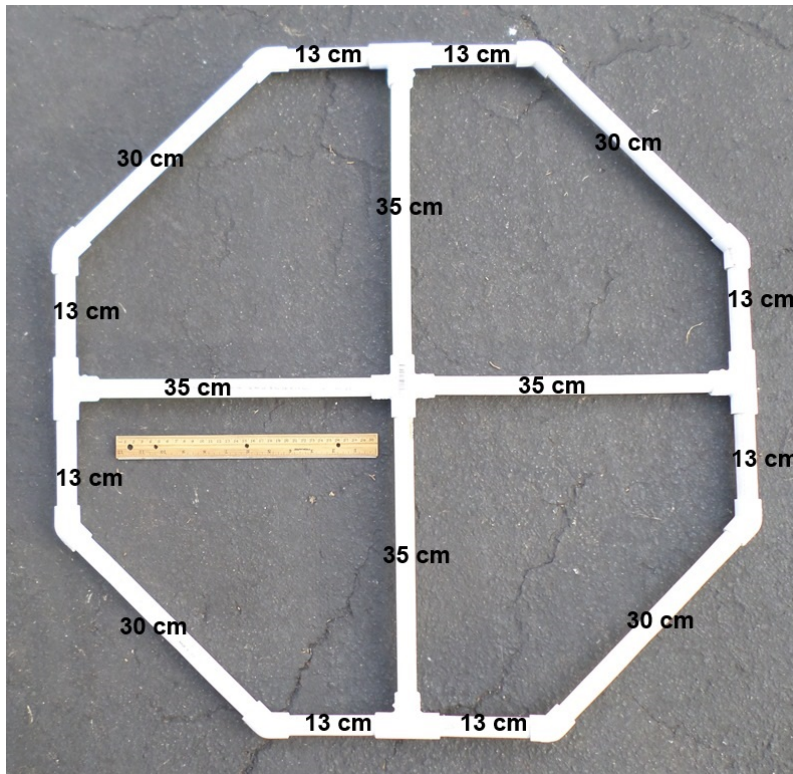
RANGER build photo #21: The paddlewheel.
