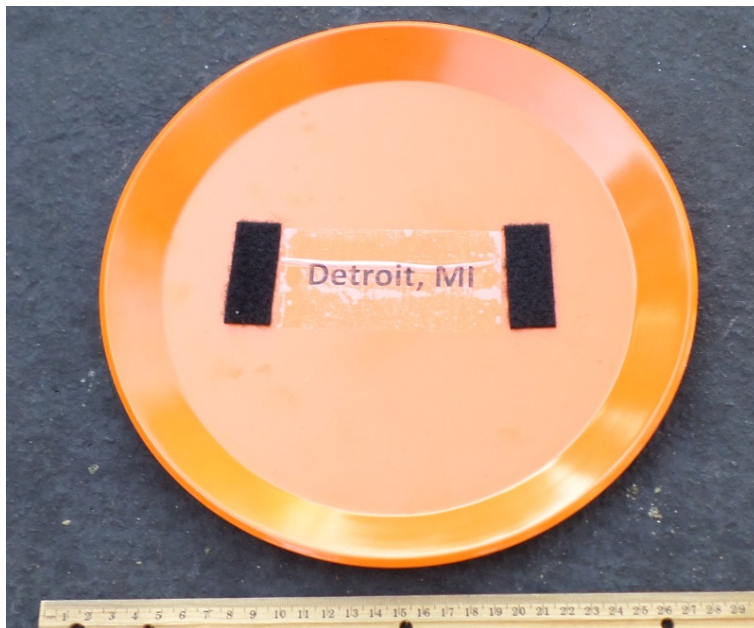
RANGER build photo #38: Ceramic plate with cover off.
