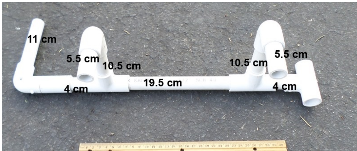
RANGER build photo #30: Locking mechanism for the cargo container.
