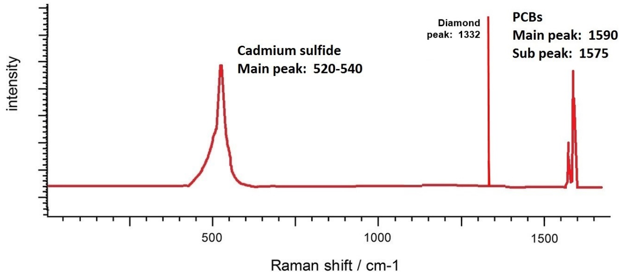
Raman spectrum of sediment contaminated with CdS (520-540 \text{cm}^{-1} ) and PCBs (1590 and 1575). Note the diamond peak (1332 \text{cm}^{-1} ).
