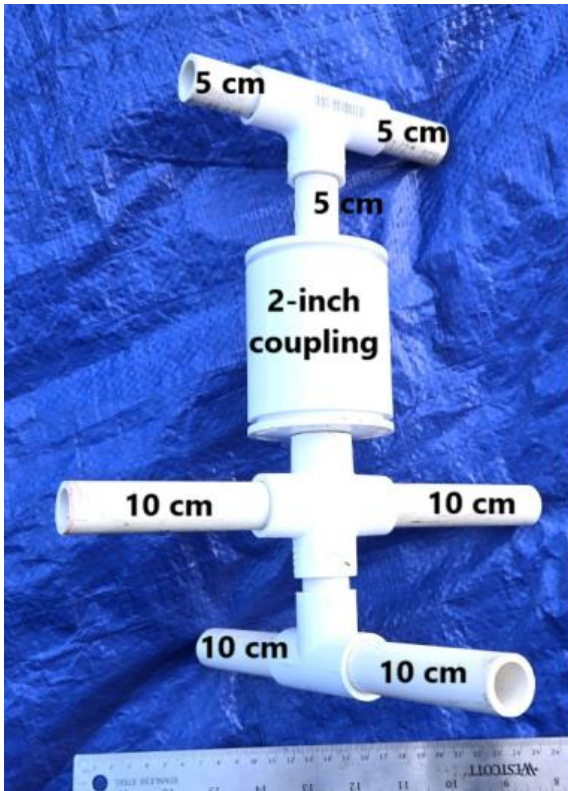
Both the old and the new sacrificial anode are constructed from 2-inch and \frac{1}{2} -inch PVC pipe. Left: The anode. Right: The anode painted silver.
