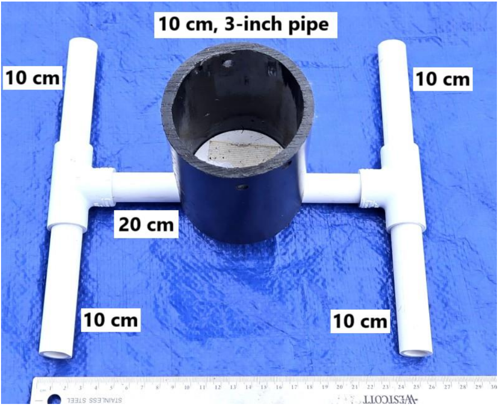
The base of the hydrophone is constructed from \frac{1}{2} -inch PVC and 3-inch pipe. Two \frac{1}{4} -inch holes are drilled across from each other in the 3-inch pipe, 1 cm from the top edge.
