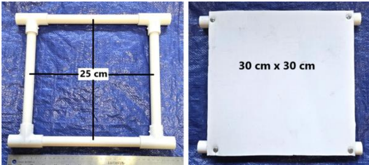
The hydrophone platform is constructed from ½-inch PVC pipe and corrugated plastic.
