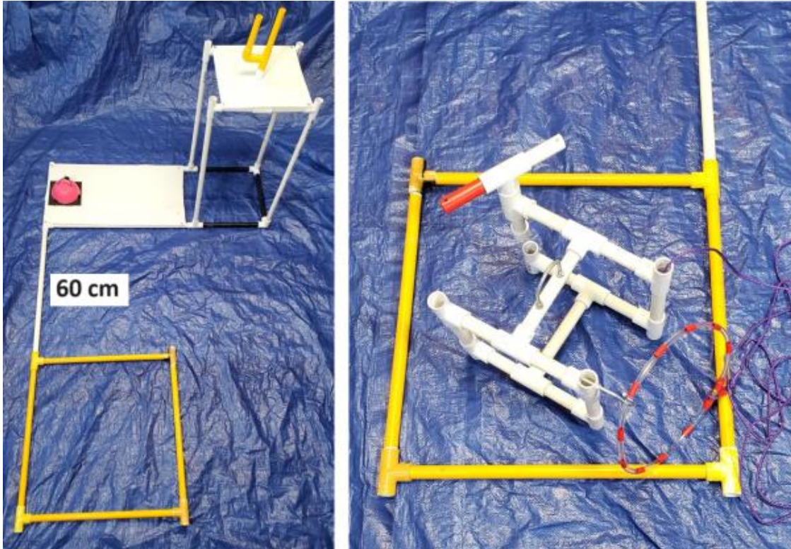
Left: The coral restoration area with the irrigation system designated area attached. Right: The irrigation system successfully deployed in the designated area.
