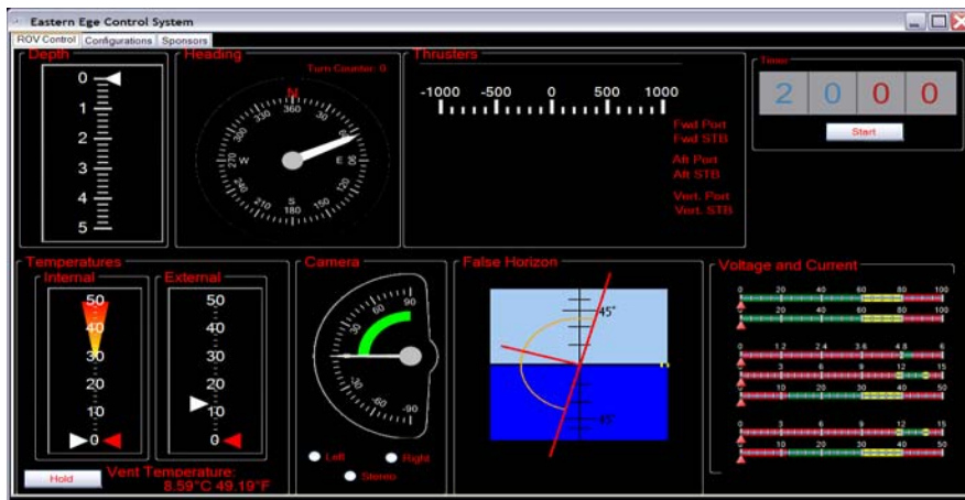
Figure 7. ROV Control Tab
