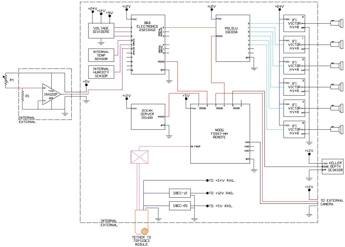
Figure B2. Schematic for submarine electronics
