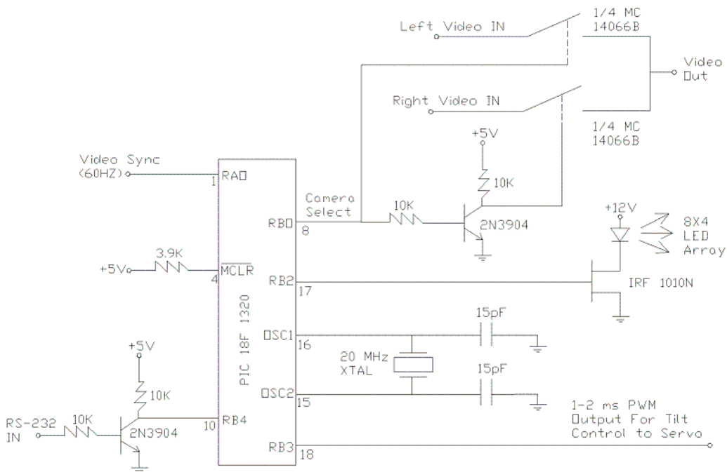
Figure B3. Electronic schematic for stereo camera
