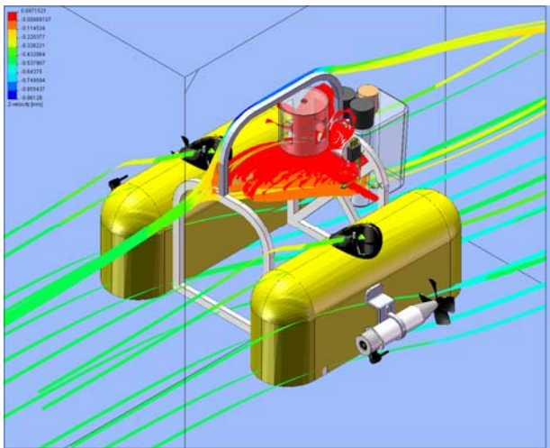
Figure A1. Flow trajectory of fluid particles as the ROV surges forward at 0.5 m/s:
