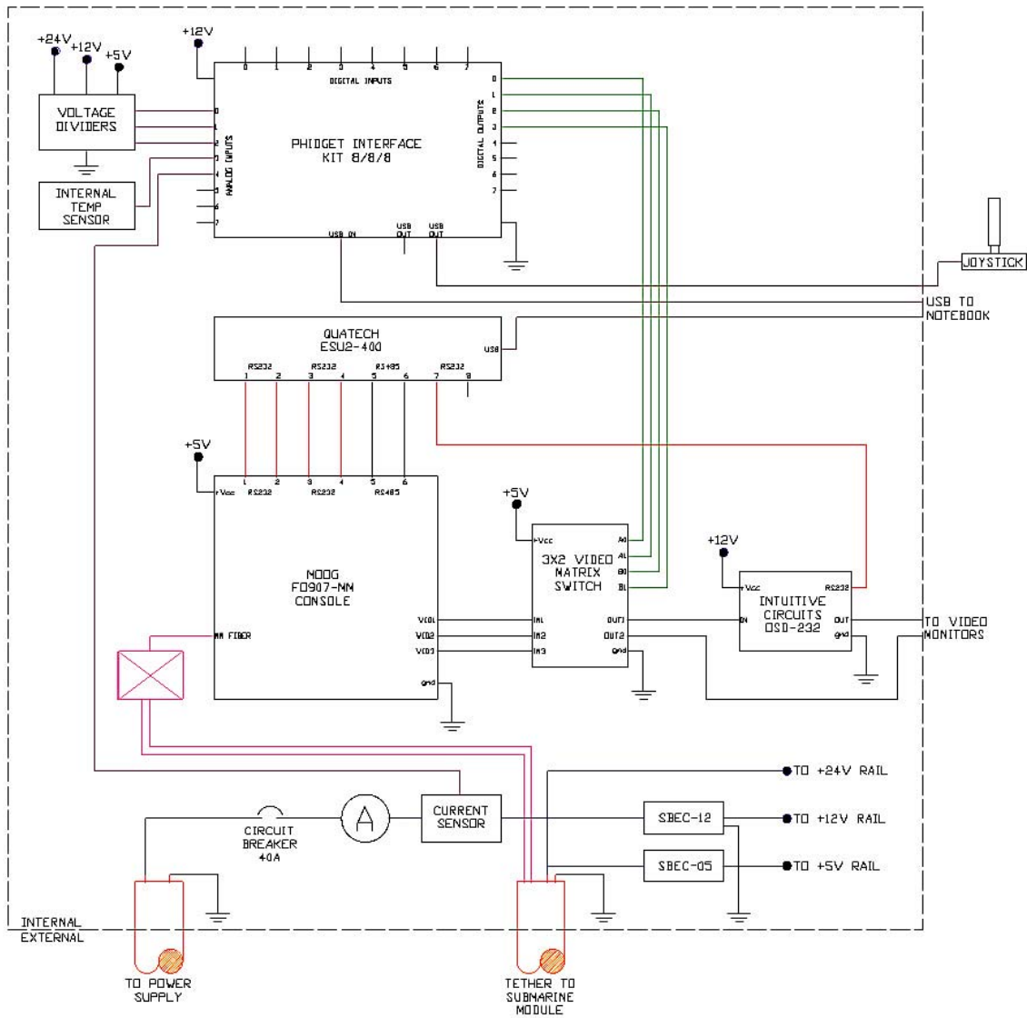
Figure B1. Schematic for topsides electronics
