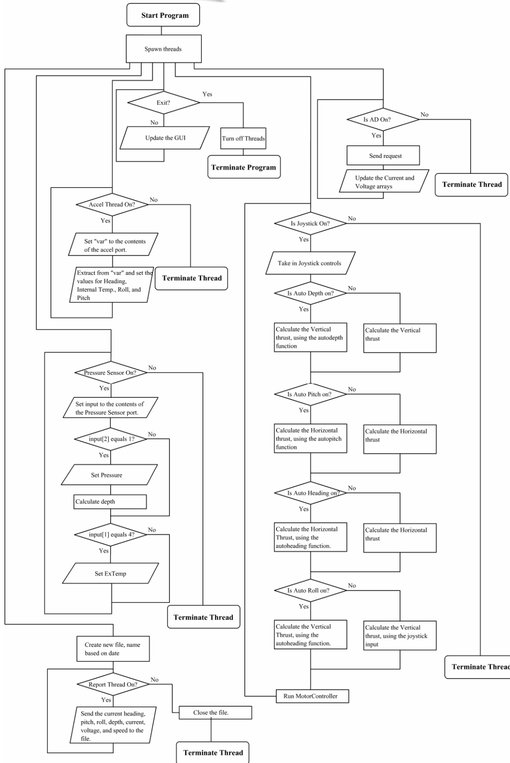
Figure 6. Programming flowchart
