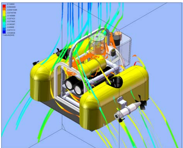
Figure A2. Flow trajectory of the fluid particles as the ROV/OBS rises at 0.5 m/s:
