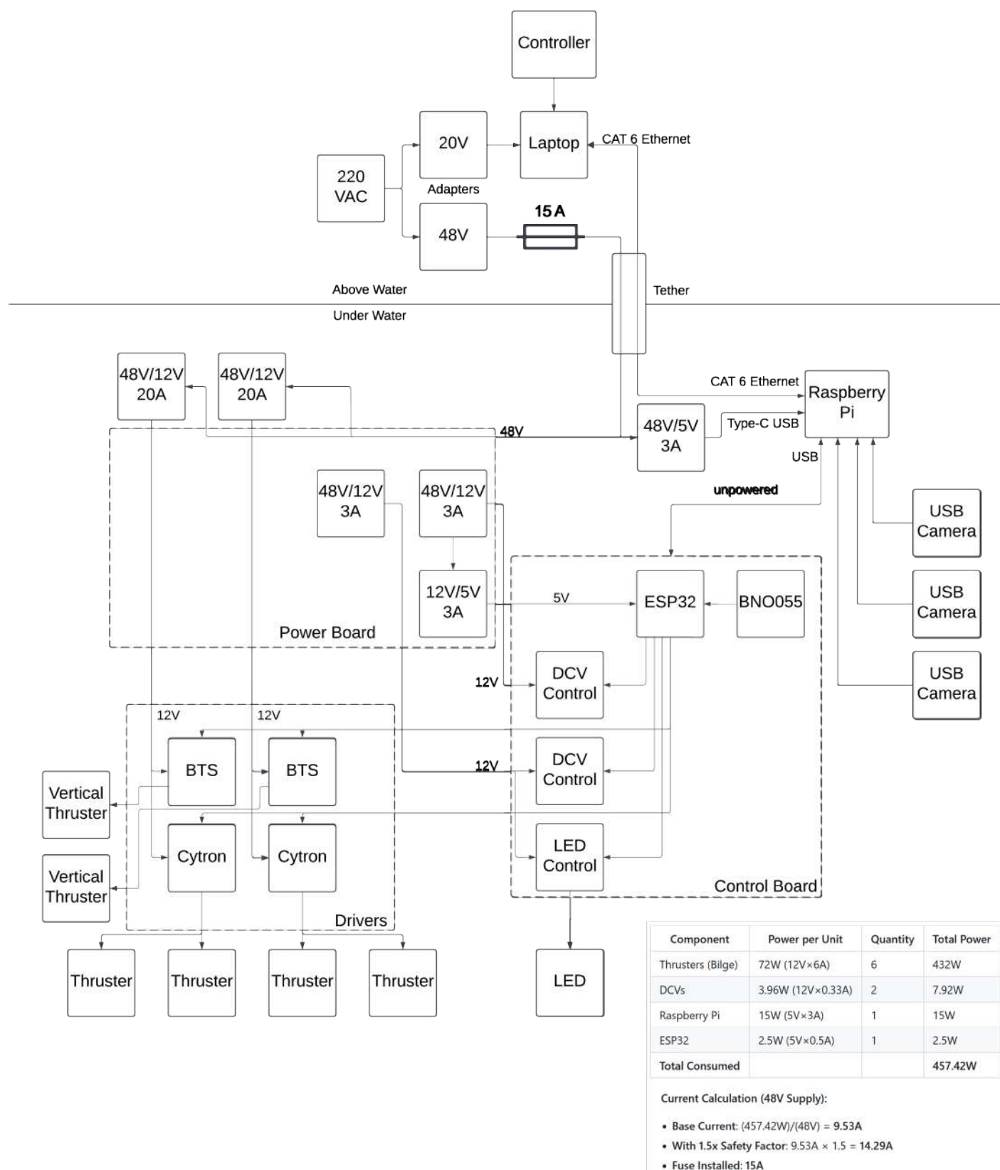
Figure 36: Electric System Interface Diagram (SID).
