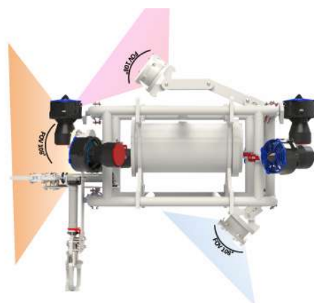
Figure 22: Cameras' FOVs.
