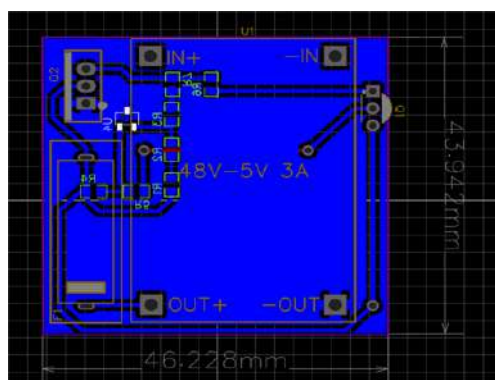
Figure 20: Overvoltage Protection Board.
