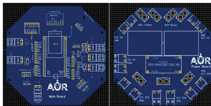
Figure 4: PCB Design
